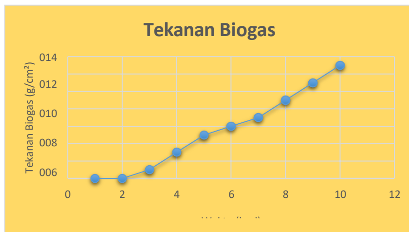
Picture 13. Biogas Pressure Inside The Digester
