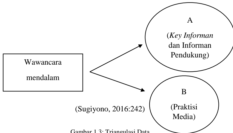
Gambar 1.3: Triangulasi Data
