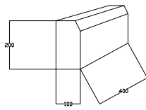
DETAIL KANSTIN SKALA 1:
