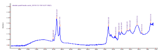
Figure 6. FTIR spectra revealing phenolic groups in Ferulic Acid isolate from rice bran oil.
