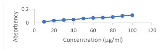
Figure 4. Wavelength calibration curve using Ferulic Acid standards at 765 nm.
