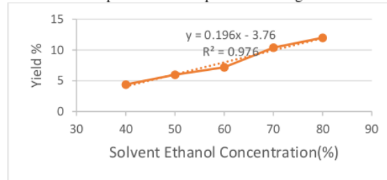
Figure 3. Correlation curve between FA yields and ethanol concentrations.
