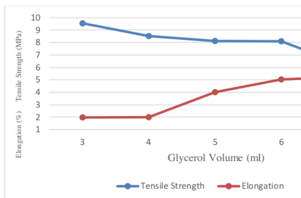
Figure 3. Glycerol Variable Tensile Strength and Elongation Test Results
