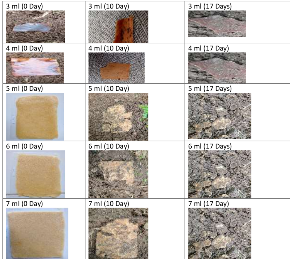
Figure 4. Biodegradation Test Results for Varying Glycerol Volume
